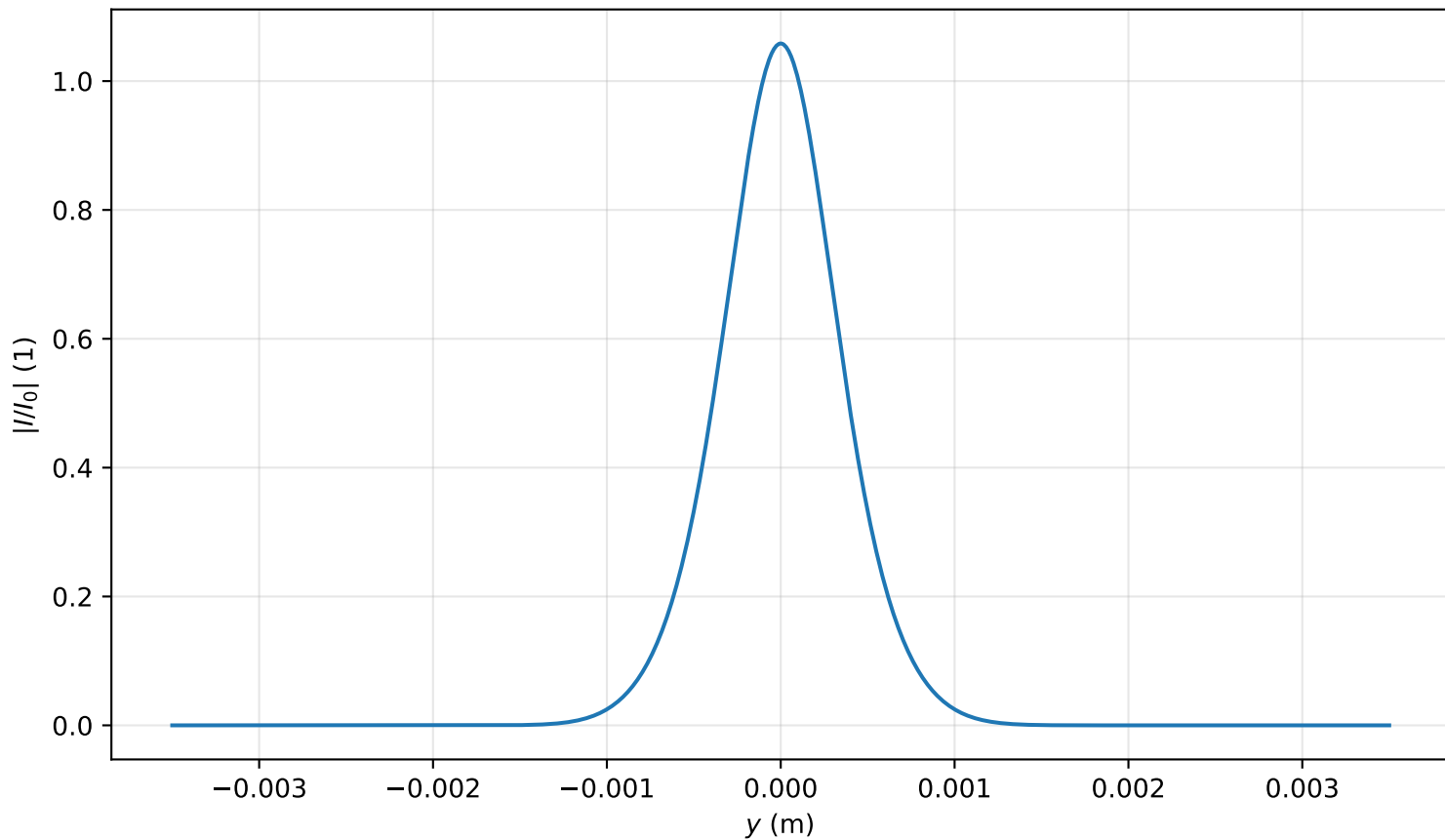
Intensity profile I(x=0, y, z=0.876)/I_0 , \text{Pin}=0.5\text{Pcr} , artificial time
